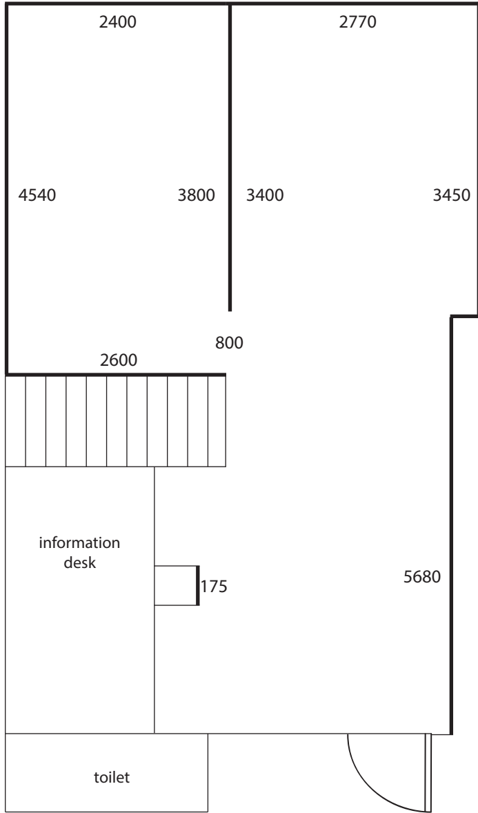
1F Height 2870
